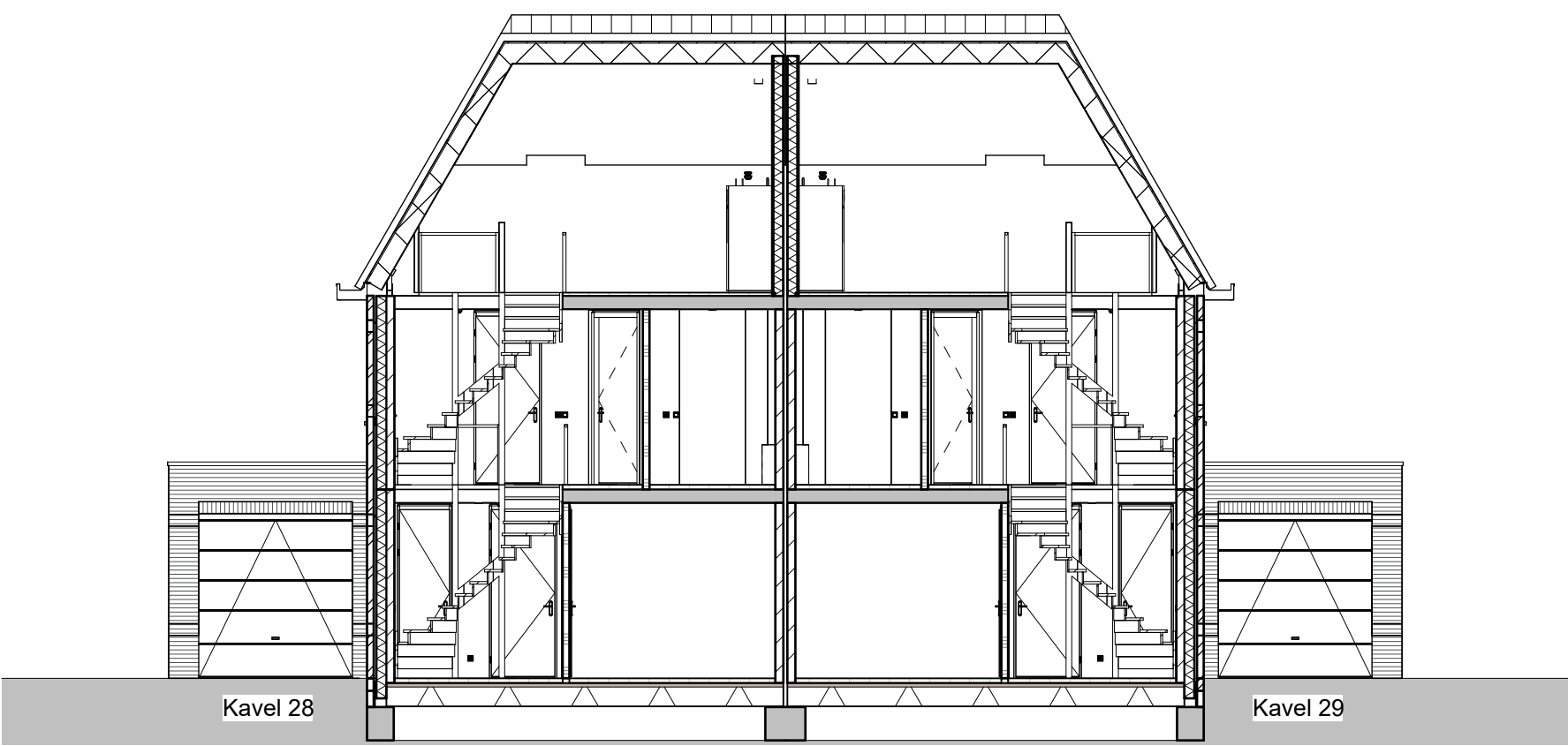
Doorsnede A_Kavel 28/29
